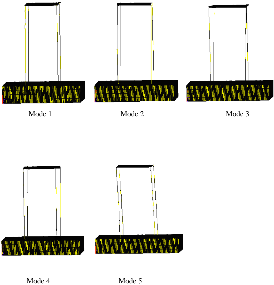
Fig 4.5 Mode shapes of simplified berthing structure with soil mass
