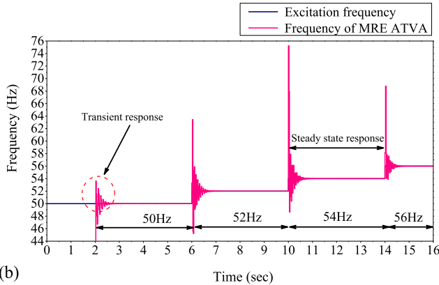
Figure 16. Simulated responses at variable frequency excitation: (a) acceleration of primary mass and (b) frequency of MRE ATVA.
