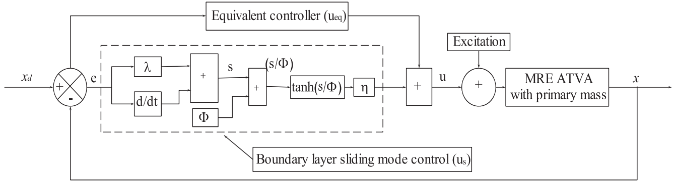
Figure 7. Schematic of boundary layer sliding mode control.
