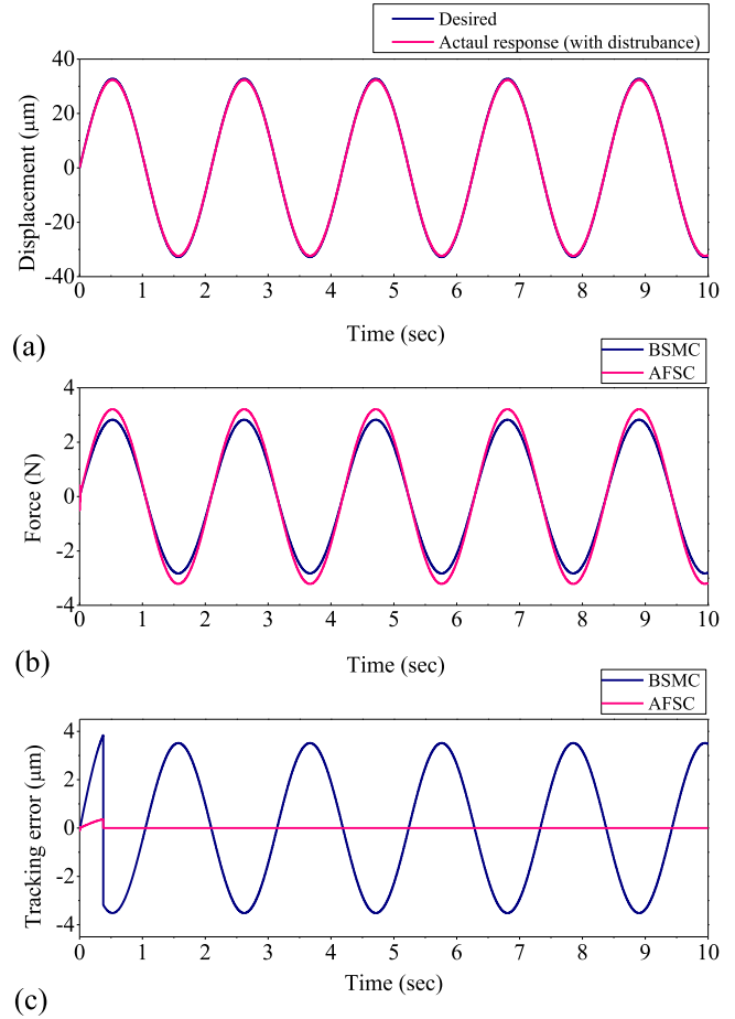
Figure 11. Time response of (a) position tracking of adaptive fuzzy sliding mode control with disturbance, (b) force with disturbance and (c) tracking error with disturbance.
