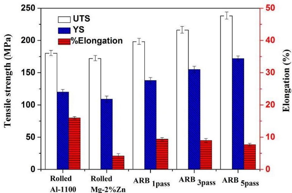
Figure 4.83. Variation of UTS, YS and percentage elongation of the Mg-2%Zn/Ce/Al hybrid composite hybrid composite with different ARB passes.
